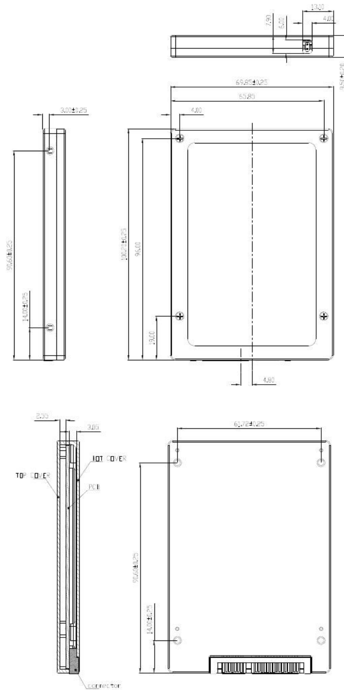
Figure 2-2. 2.5" SSD Dimensions (optional 9.5mm chassis for 1TB)
