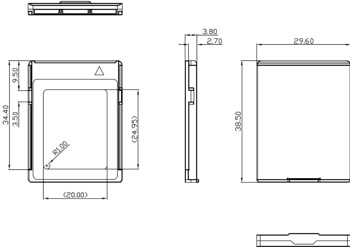
2-1. CFexpress Card Type B Dimensions
